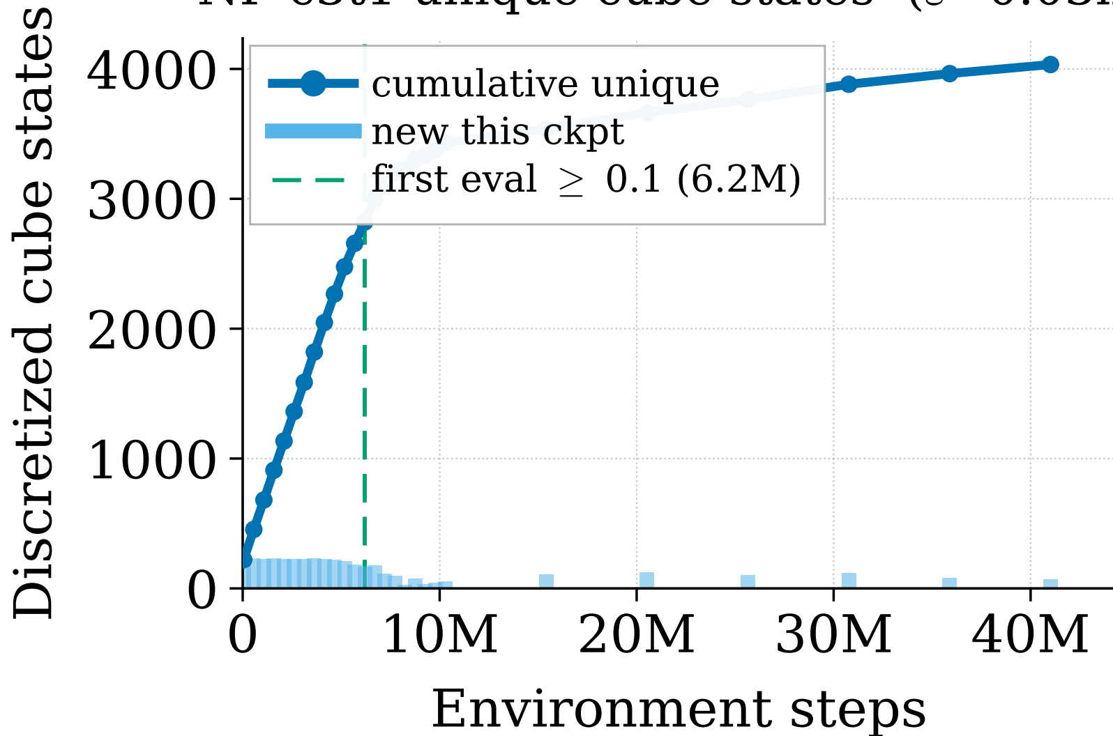
NF c3t1 unique cube states ( \varepsilon=0.03m )
